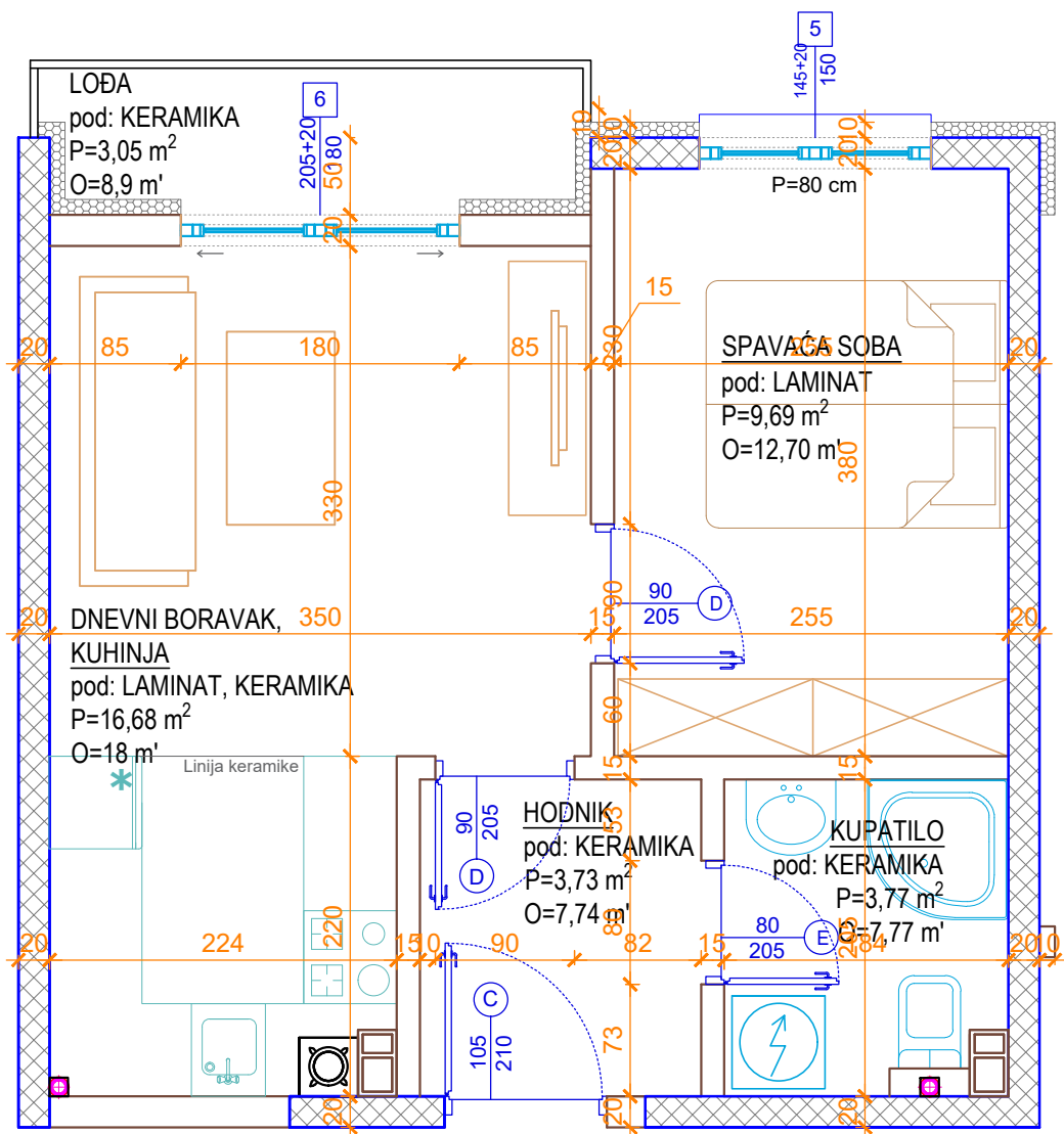
STAN 6,10,14,18 P=36,16m 2
